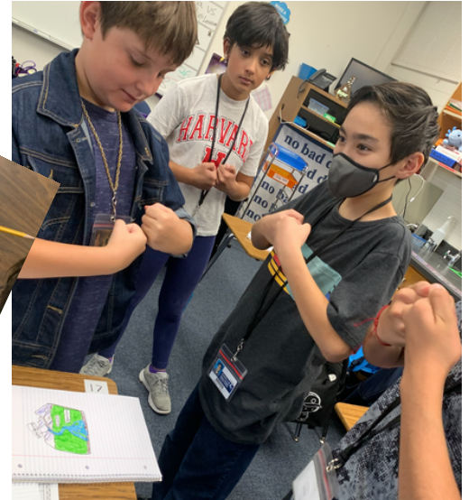
Explaining erosion, weathering, and decomposition using hand signals at Cholla Flex.
